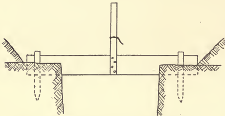
FIG. 5.—METHOD OF SETTING GRADE-PLANK.
